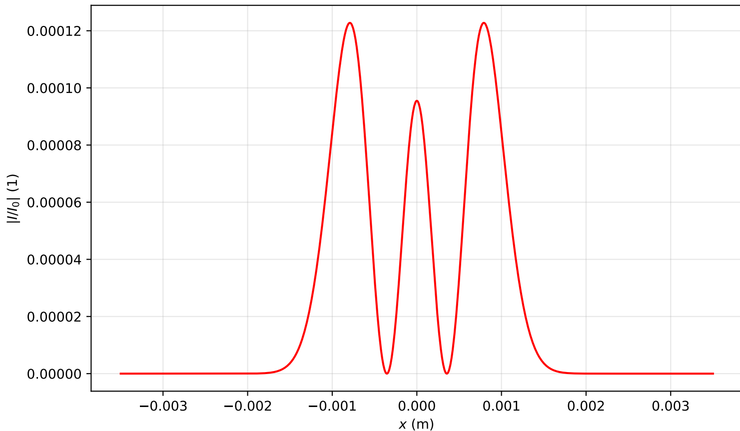
Intensity profile I(x, y = 0, z = 0.318)/I_0 , P_{in}=0.5P_{cr} , artificial time
